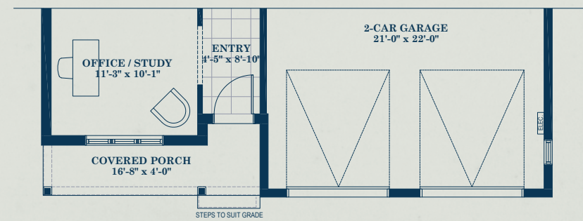
Elevation B Main Level, 1,176 sq ft
