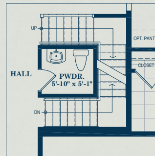
With finished lower level option elev. A & B
