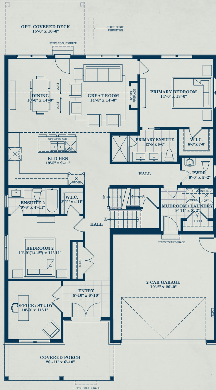
Elevation A with Loft Main Level, 1,751 sq ft
