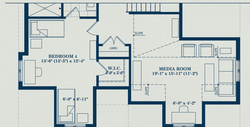
Elevation A & B with Loft & Media Room Upper Level, 1,149 sq ft
