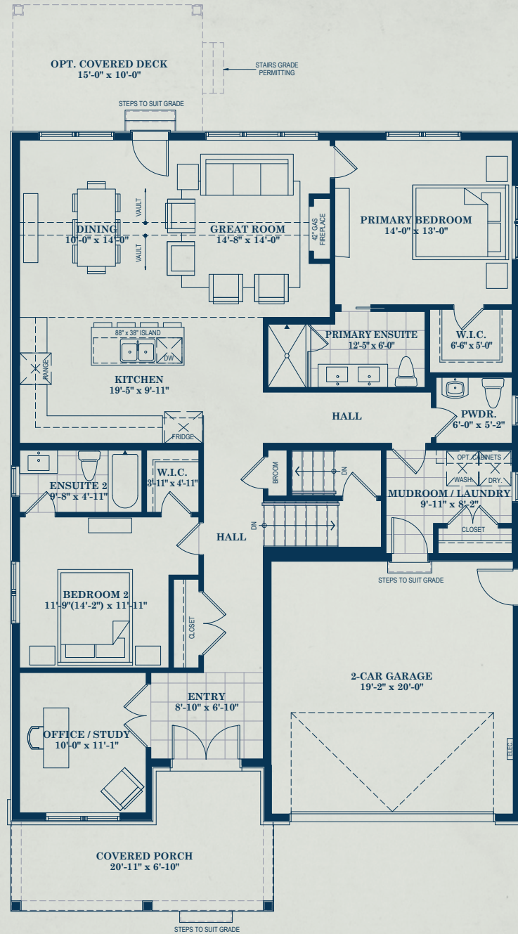
Elevation A Main Level, 1,751 sq ft
